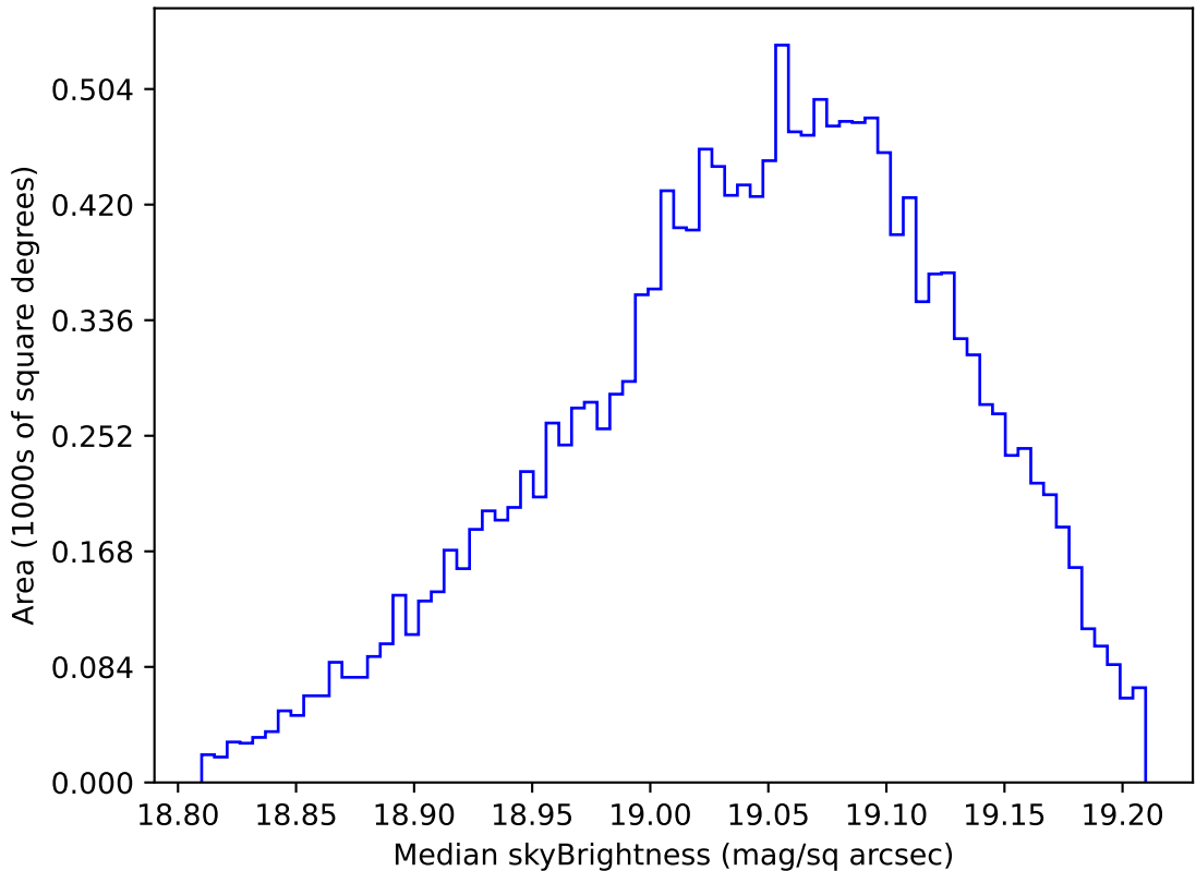
too_elab_r8_d2_giz_v3.4_10yrs WFD z band: Median skyBrightness
