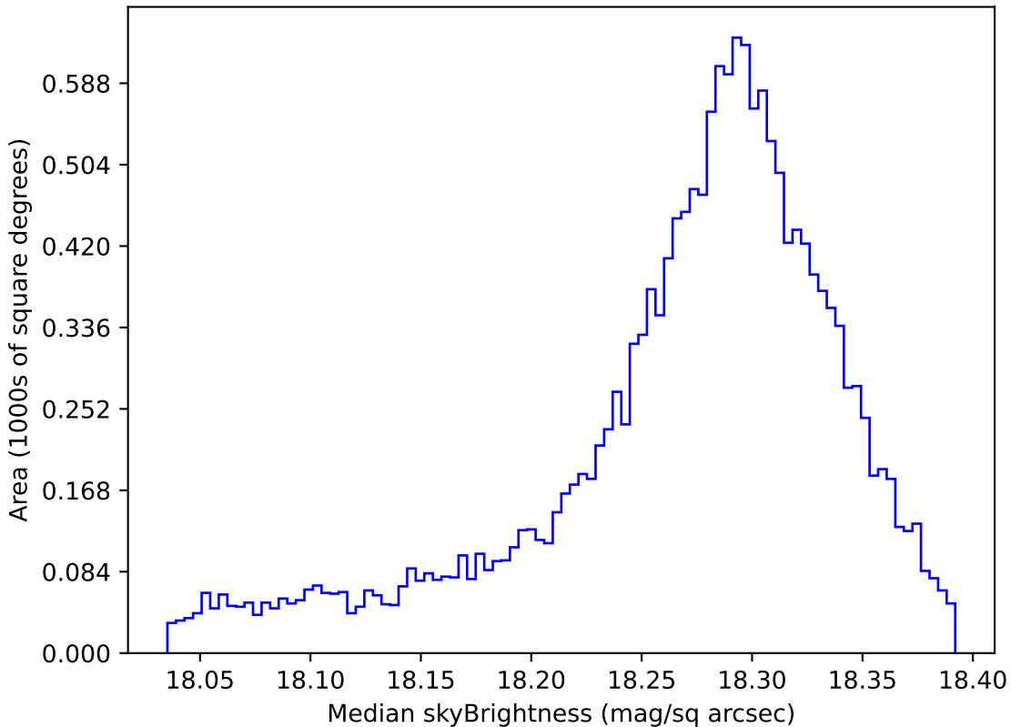
too_elab_r8_d2_giz_v3.4_10yrs WFD y band: Median skyBrightness
