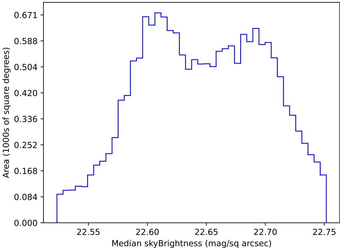
too_elab_r8_d2_giz_v3.4_10yrs WFD u band: Median skyBrightness
