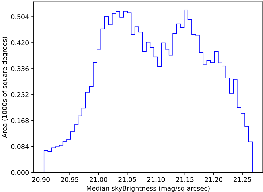
too_elab_r8_d2_giz_v3.4_10yrs WFD r band: Median skyBrightness
