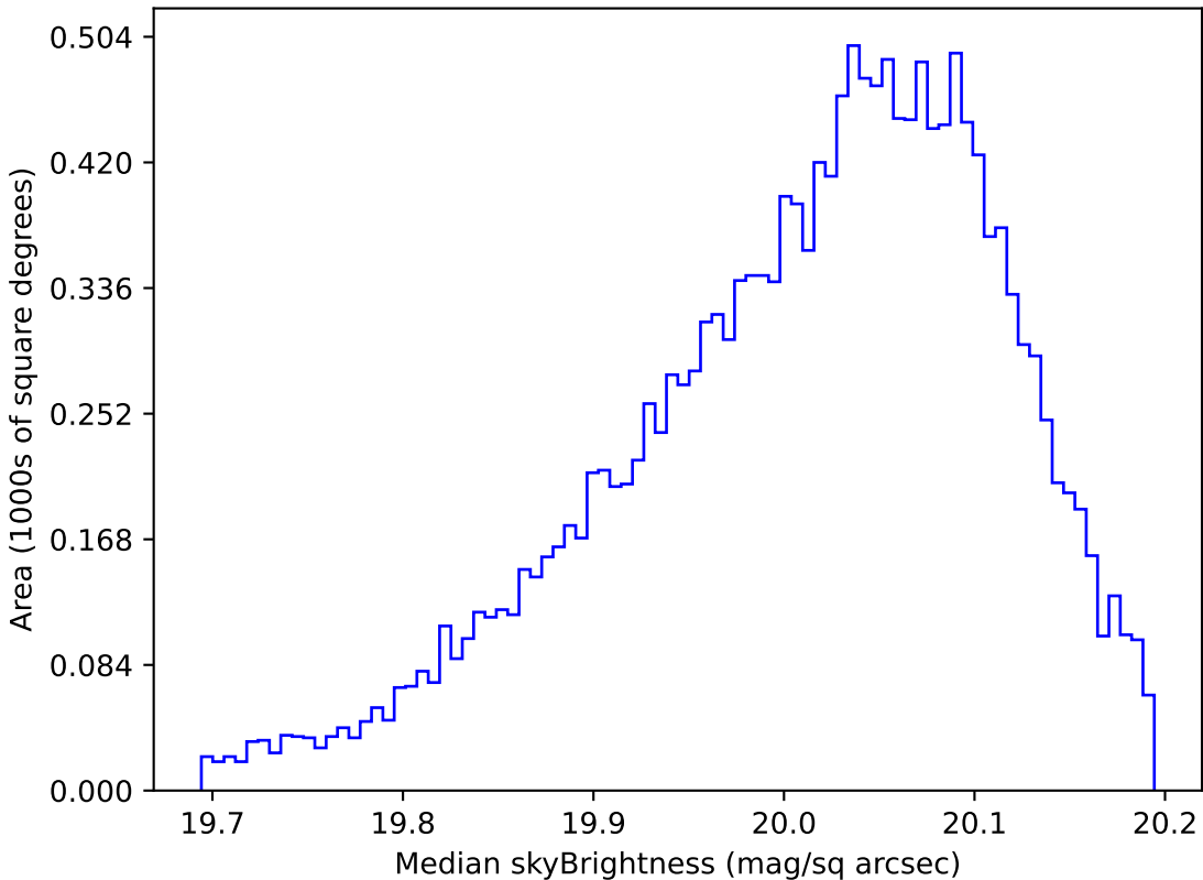
too_elab_r8_d2_giz_v3.4_10yrs WFD i band: Median skyBrightness
