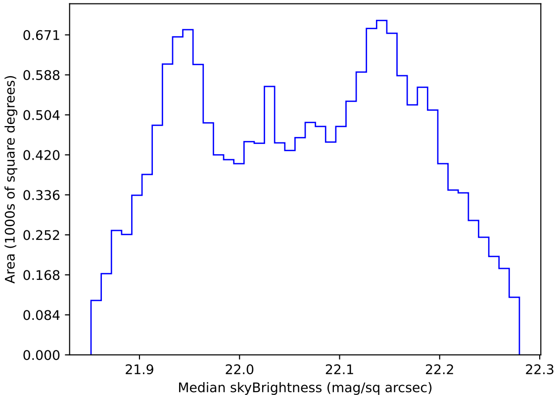
too_elab_r8_d2_giz_v3.4_10yrs WFD g band: Median skyBrightness
