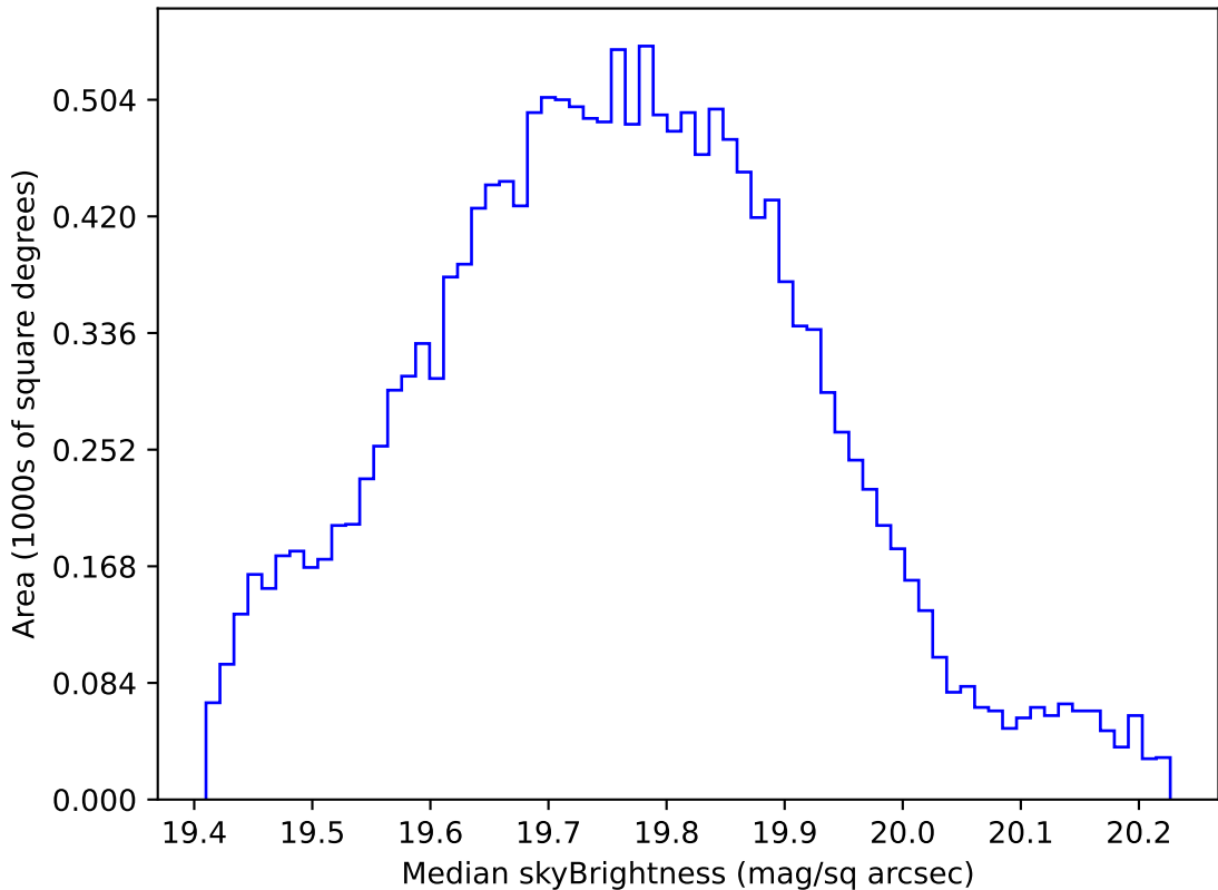
too_elab_r8_d2_giz_v3.4_10yrs WFD all bands: Median skyBrightness
