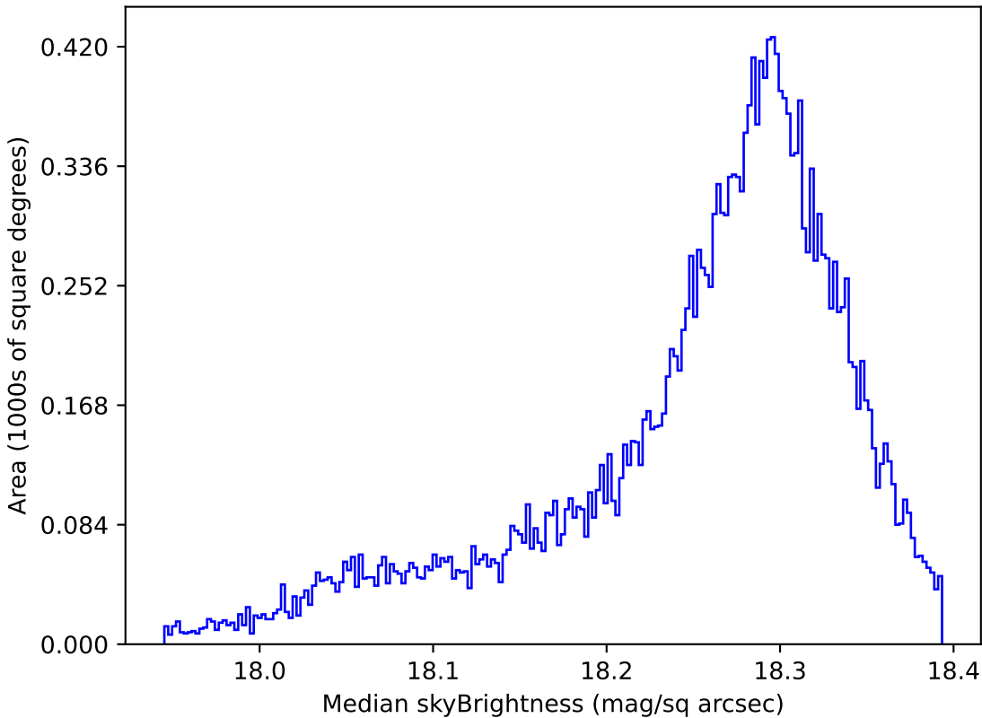
too_elab_r8_d2_giz_v3.4_10yrs All sky y band: Median skyBrightness
