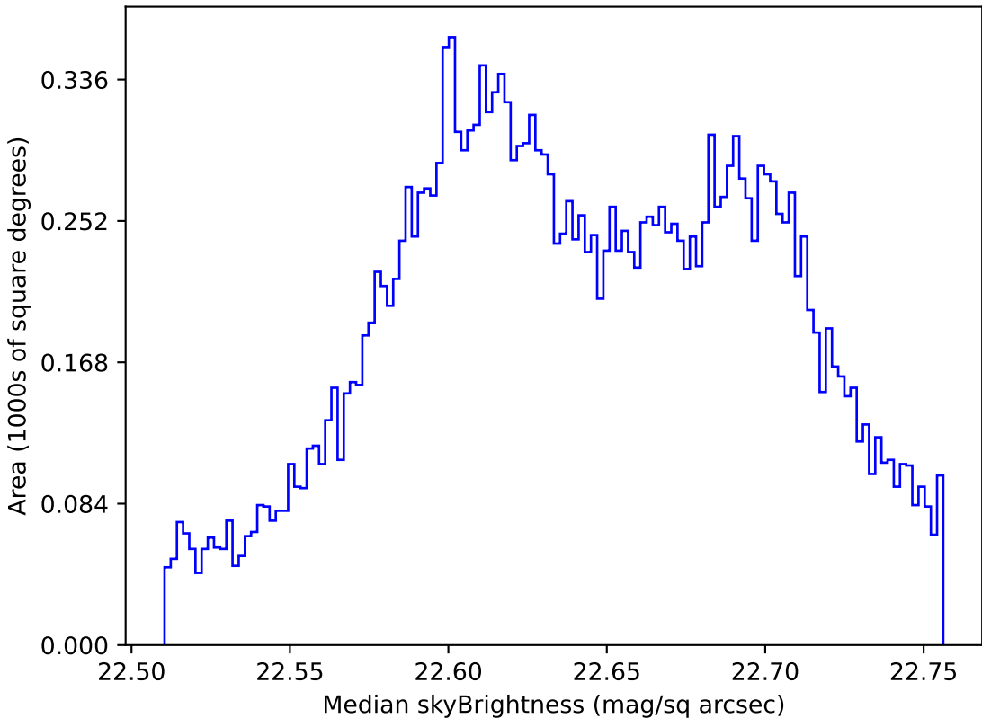
too_elab_r8_d2_giz_v3.4_10yrs All sky u band: Median skyBrightness
