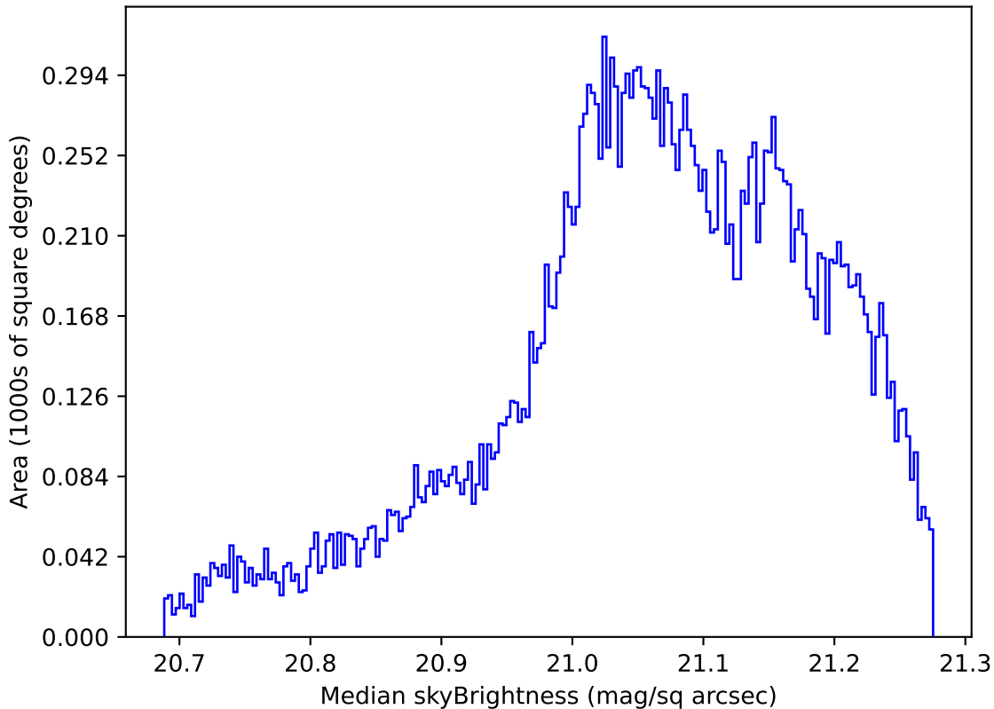
too_elab_r8_d2_giz_v3.4_10yrs All sky r band: Median skyBrightness
