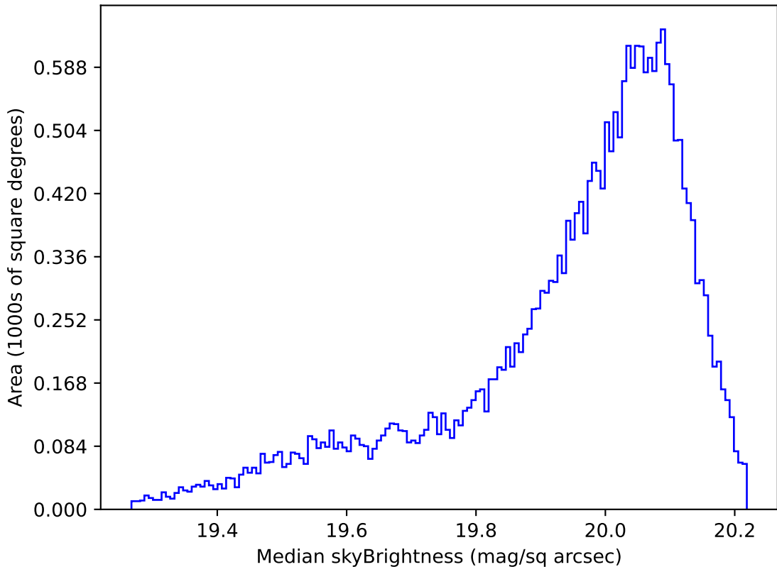
too_elab_r8_d2_giz_v3.4_10yrs All sky i band: Median skyBrightness
