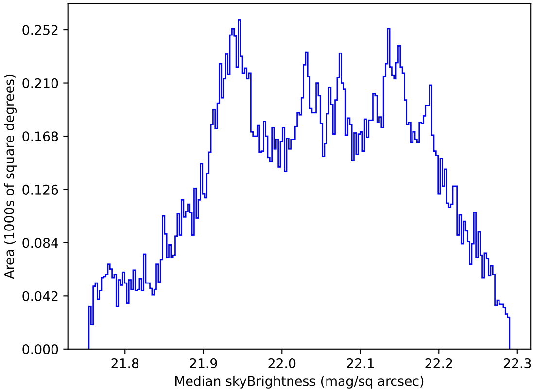
too_elab_r8_d2_giz_v3.4_10yrs All sky g band: Median skyBrightness
