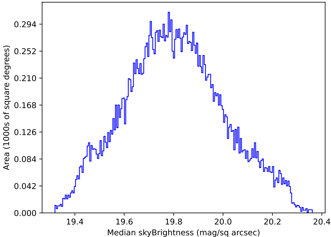
too_elab_r8_d2_giz_v3.4_10yrs All sky all bands: Median skyBrightness
