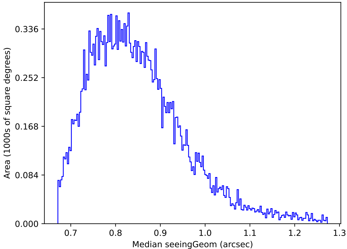
too_elab_r8_d2_giz_v3.4_10yrs Yr 1 z band: Median seeingGeom
