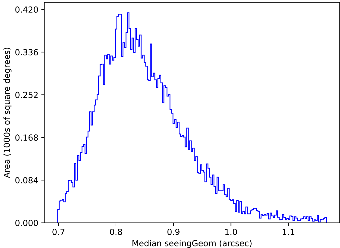
too_elab_r8_d2_giz_v3.4_10yrs Yr 1 y band: Median seeingGeom
