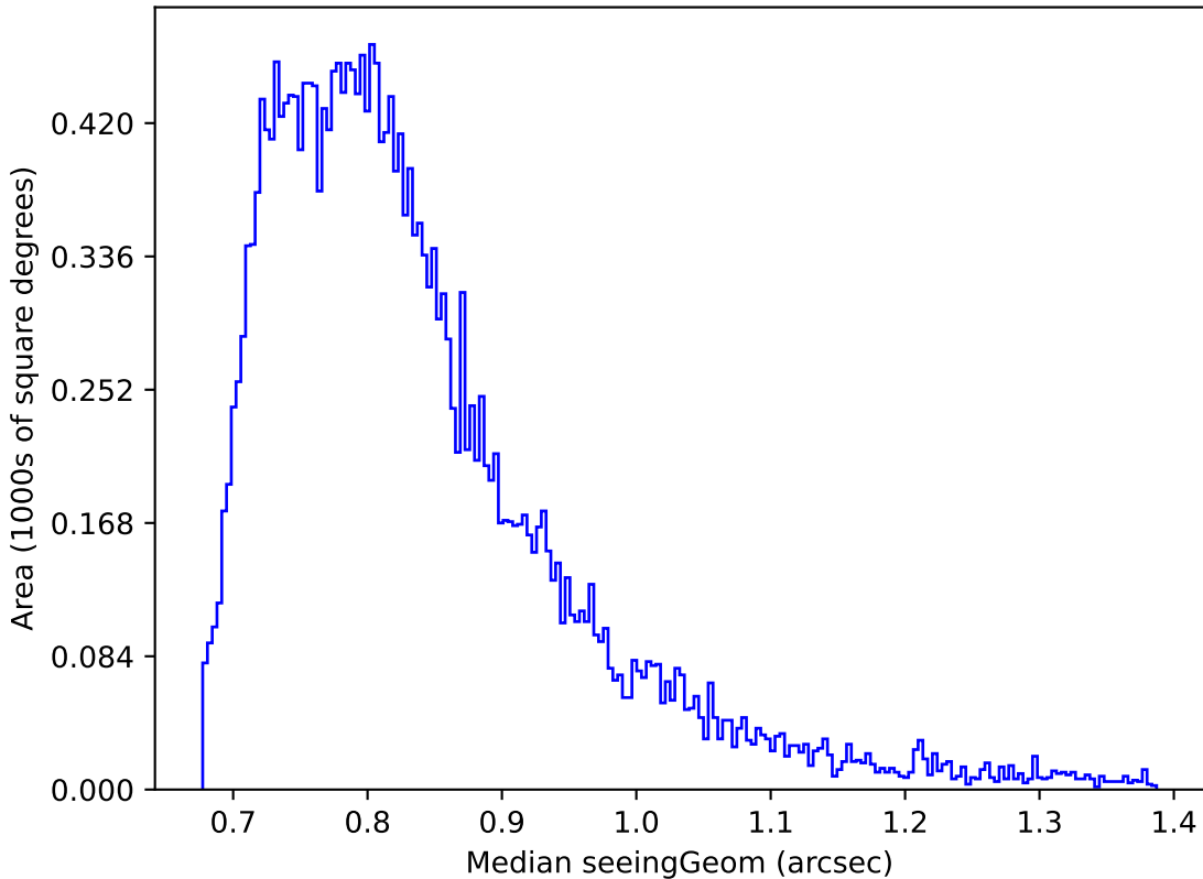
too_elab_r8_d2_giz_v3.4_10yrs Yr 1 i band: Median seeingGeom
