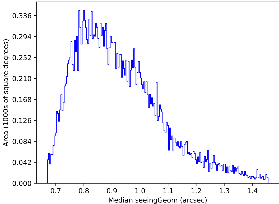
too_elab_r8_d2_giz_v3.4_10yrs Yr 1 g band: Median seeingGeom
