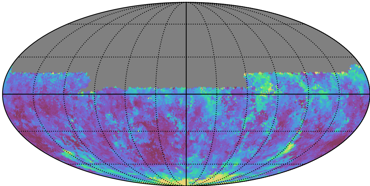
too_elab_r8_d2_giz_v3.4_10yrs Yr 1 y band: Median seeingEff
