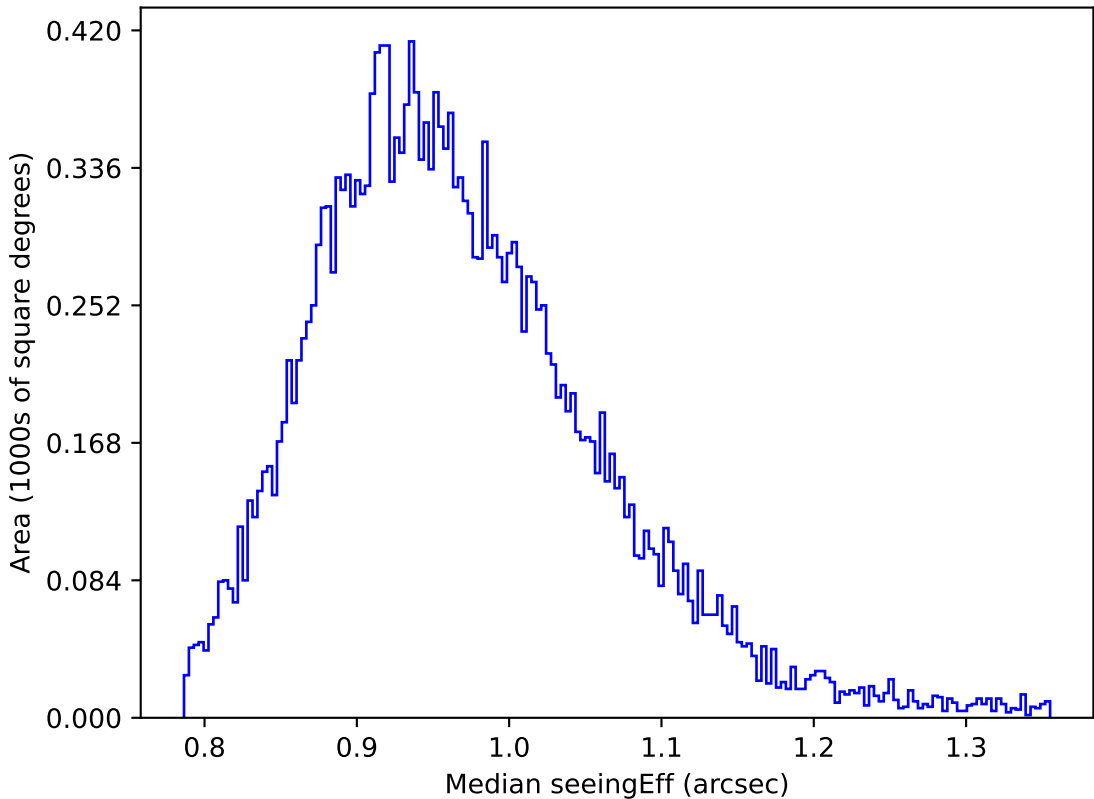
too_elab_r8_d2_giz_v3.4_10yrs Yr 1 y band: Median seeingEff
