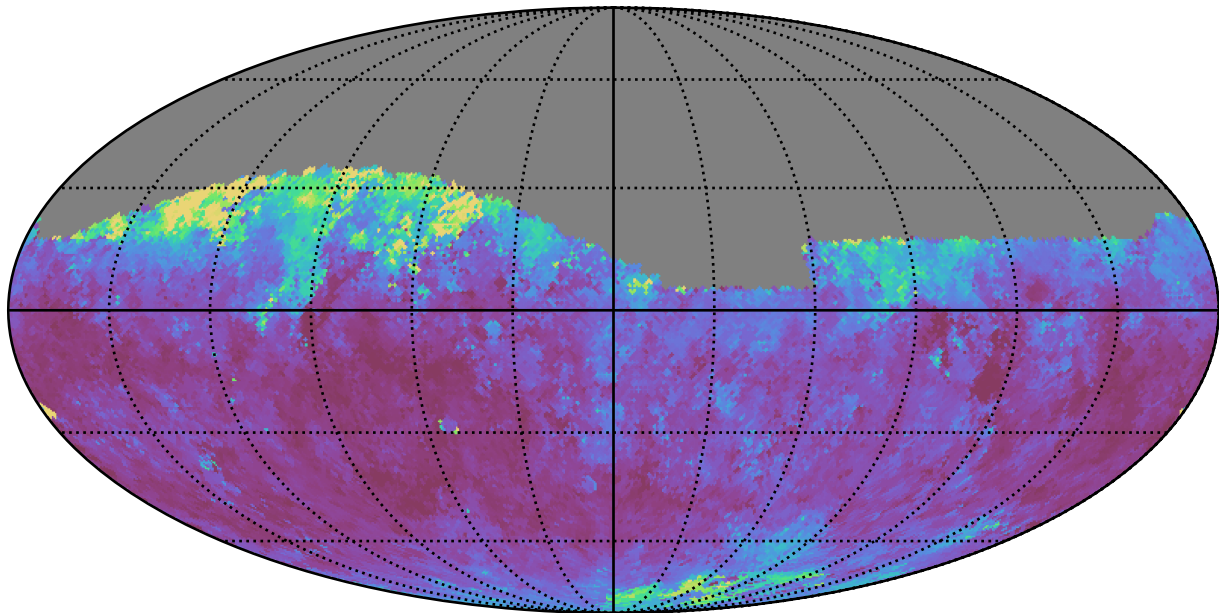
too_elab_r8_d2_giz_v3.4_10yrs Yr 1 i band: Median seeingEff
