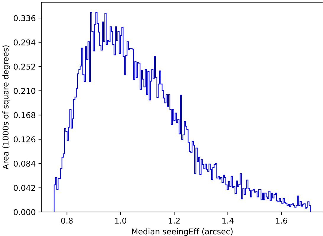
too_elab_r8_d2_giz_v3.4_10yrs Yr 1 g band: Median seeingEff
