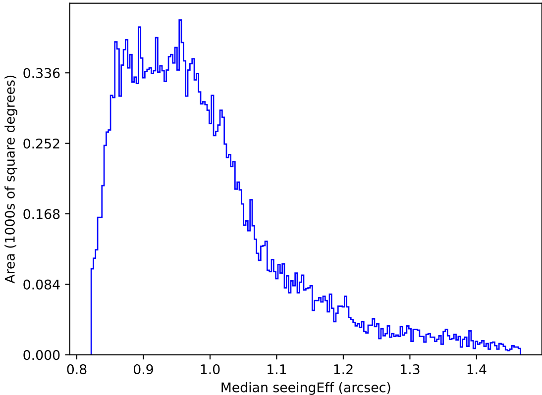
too_elab_r8_d2_giz_v3.4_10yrs Yr 1 all bands: Median seeingEff
