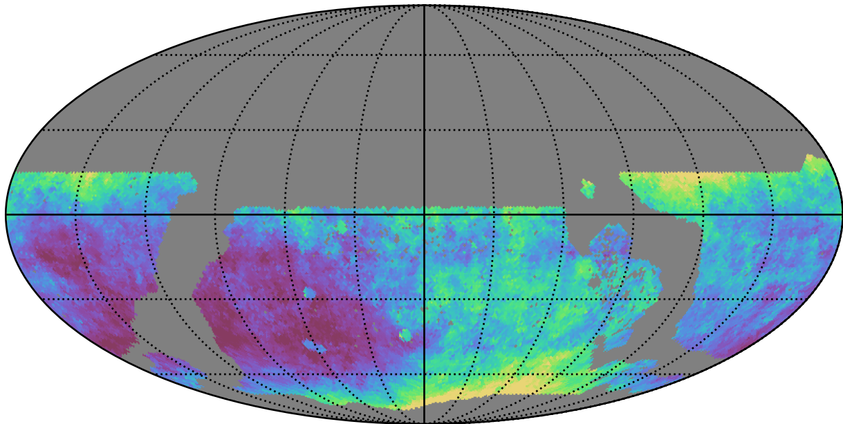
too_elab_r8_d2_giz_v3.4_10yrs WFD z band: Median seeingEff
