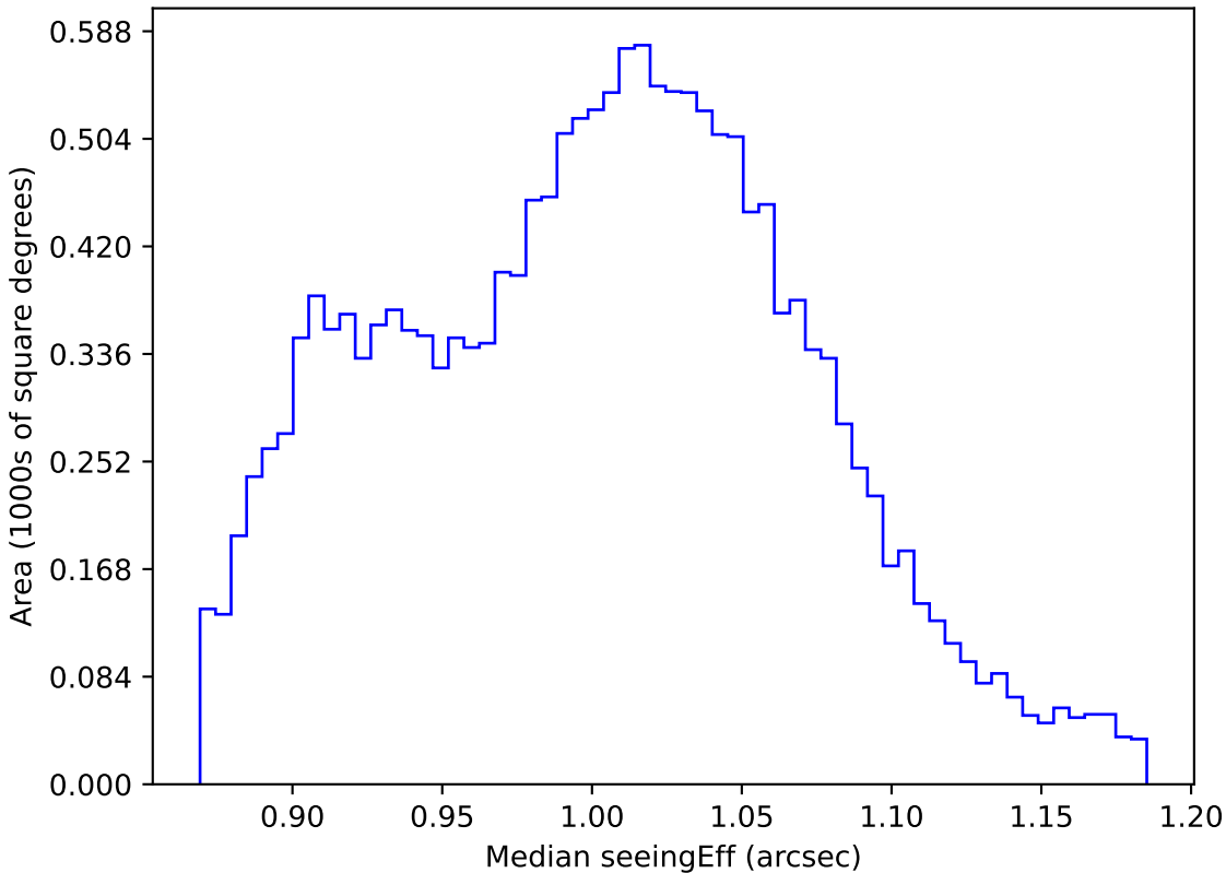
too_elab_r8_d2_giz_v3.4_10yrs WFD z band: Median seeingEff
