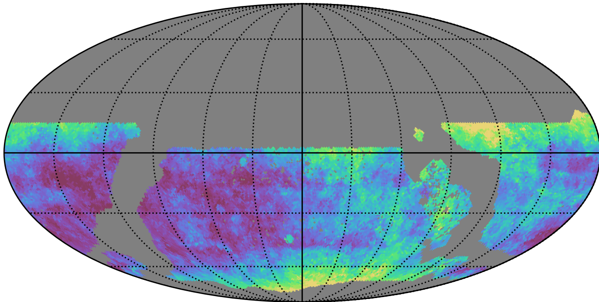
too_elab_r8_d2_giz_v3.4_10yrs WFD y band: Median seeingEff
