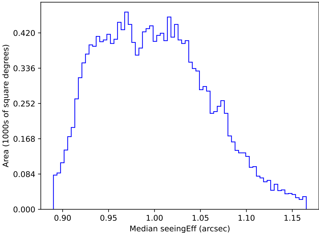
too_elab_r8_d2_giz_v3.4_10yrs WFD y band: Median seeingEff
