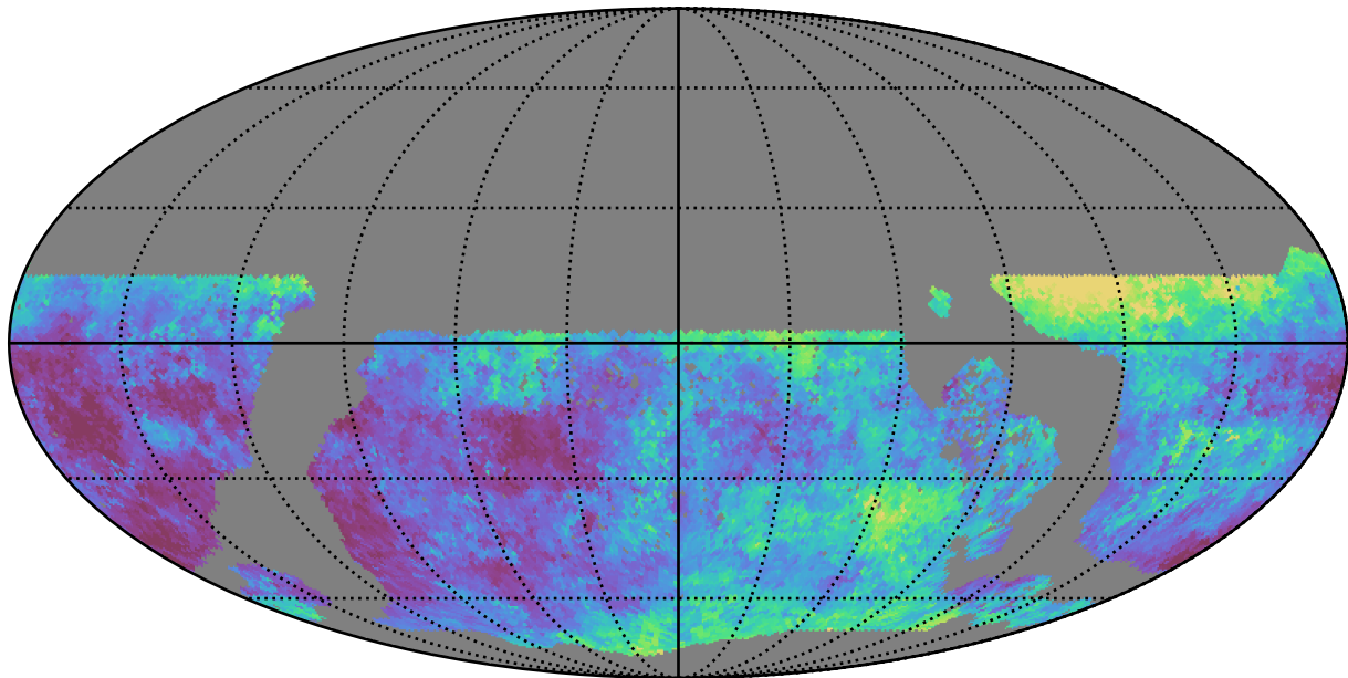
too_elab_r8_d2_giz_v3.4_10yrs WFD u band: Median seeingEff
