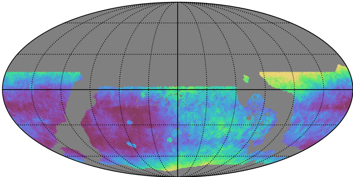
too_elab_r8_d2_giz_v3.4_10yrs WFD r band: Median seeingEff
