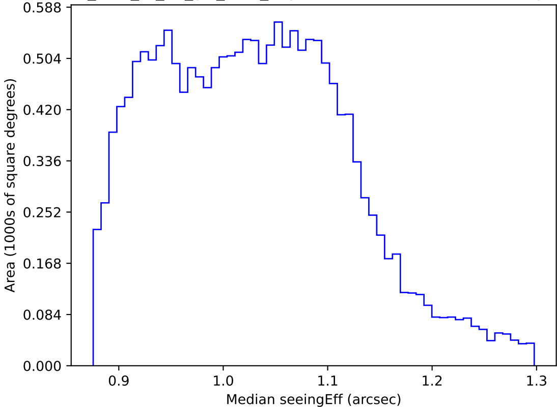
too_elab_r8_d2_giz_v3.4_10yrs WFD r band: Median seeingEff
