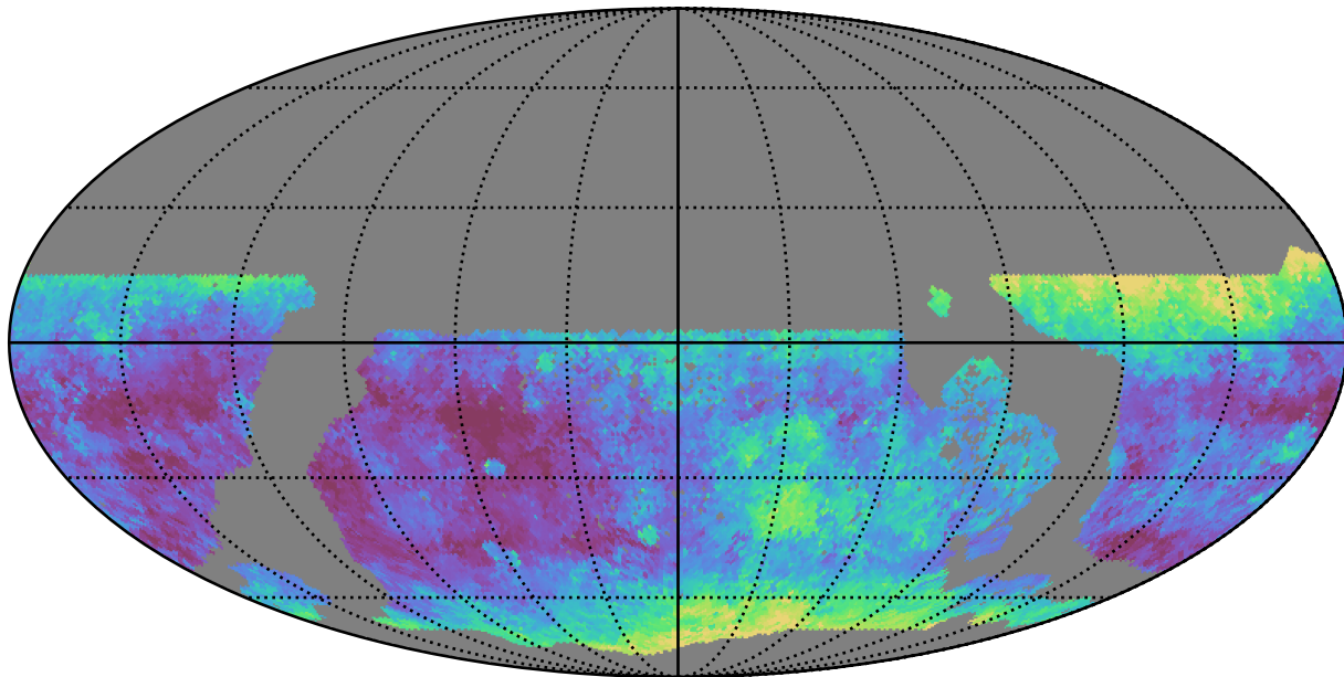
too_elab_r8_d2_giz_v3.4_10yrs WFD g band: Median seeingEff
