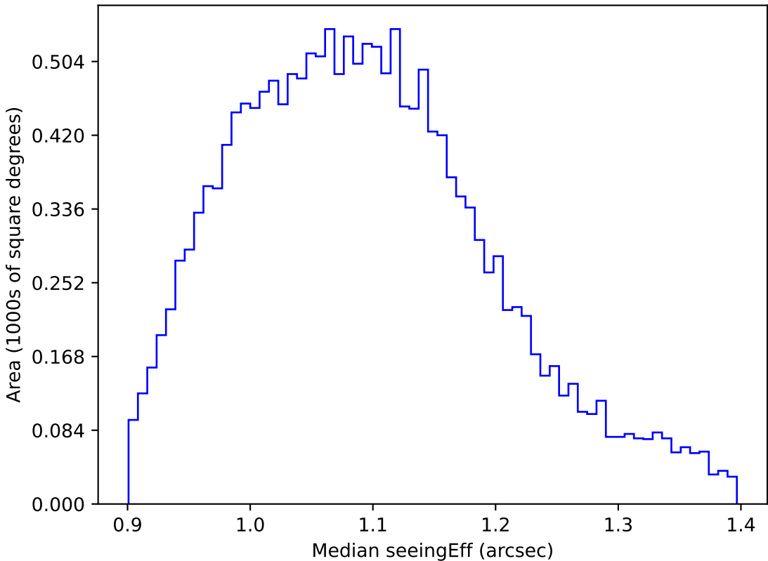
too_elab_r8_d2_giz_v3.4_10yrs WFD g band: Median seeingEff
