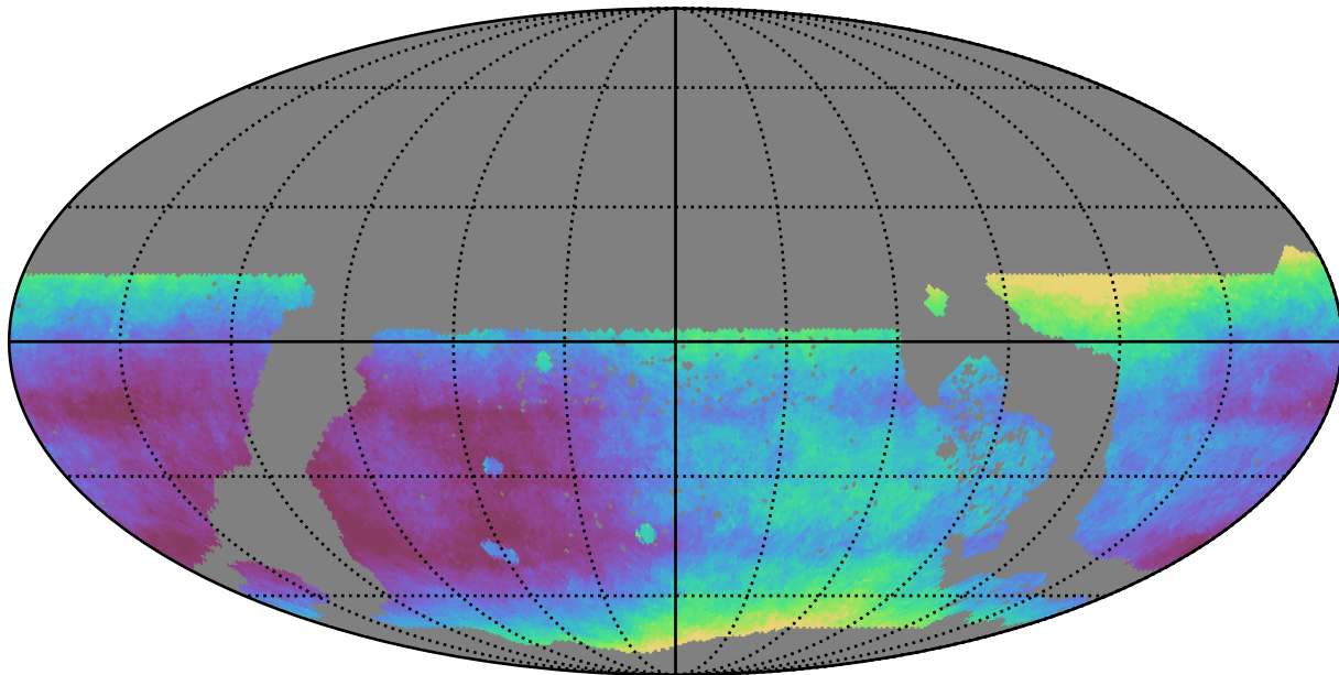
too_elab_r8_d2_giz_v3.4_10yrs WFD all bands: Median seeingEff
