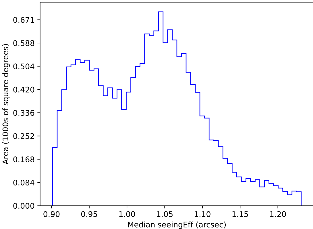
too_elab_r8_d2_giz_v3.4_10yrs WFD all bands: Median seeingEff
