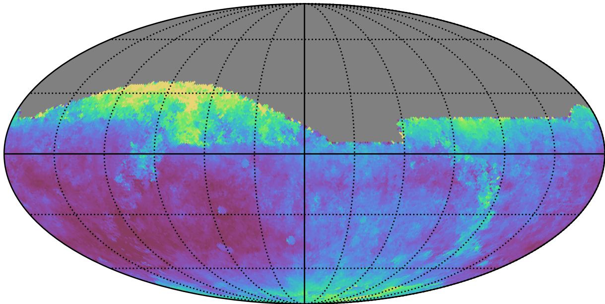
too_elab_r8_d2_giz_v3.4_10yrs All sky z band: Median seeingEff
