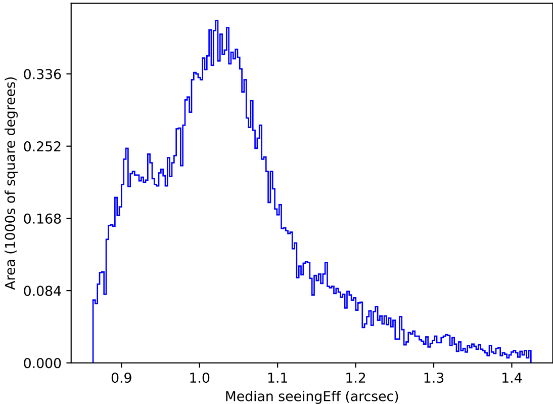
too_elab_r8_d2_giz_v3.4_10yrs All sky z band: Median seeingEff
