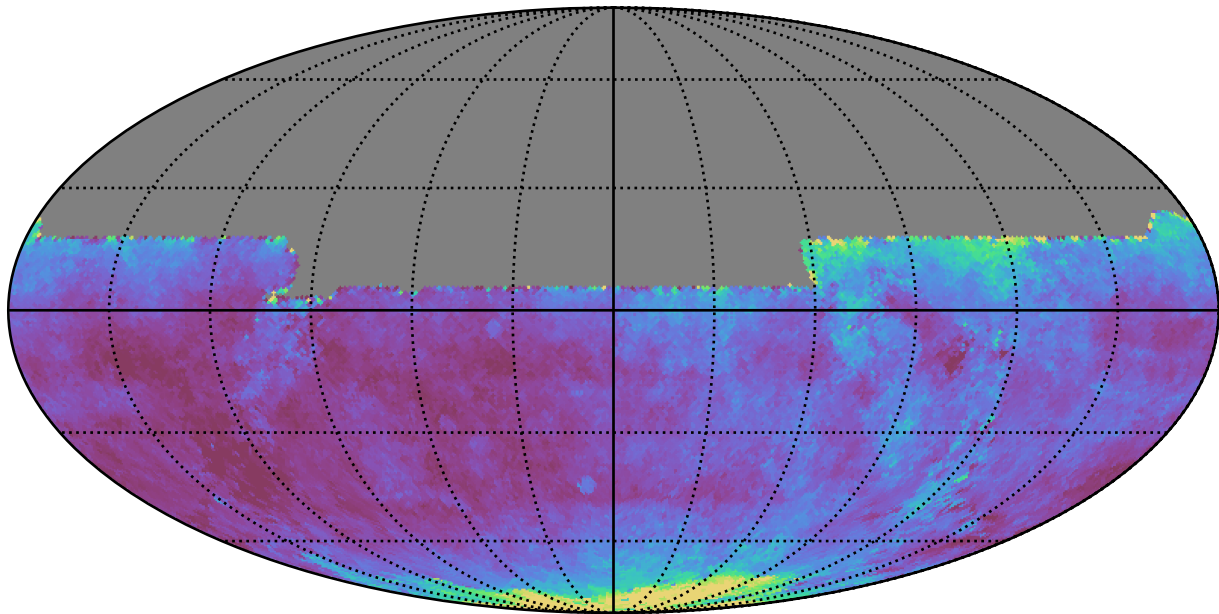
too_elab_r8_d2_giz_v3.4_10yrs All sky y band: Median seeingEff
