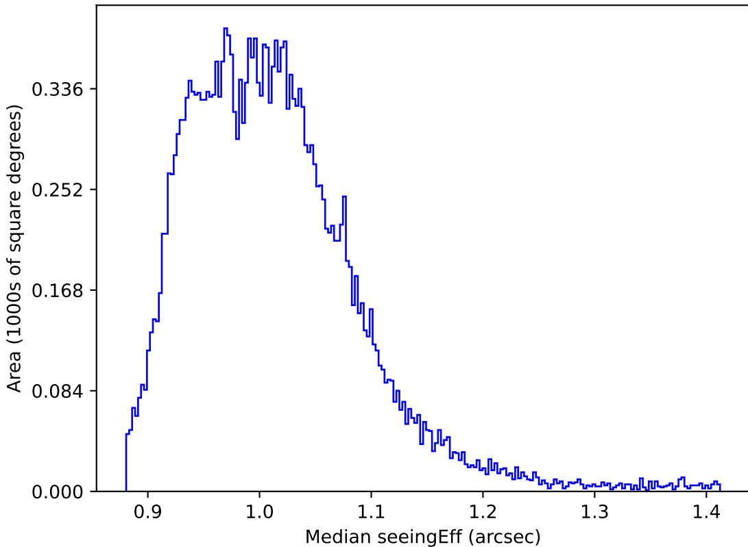
too_elab_r8_d2_giz_v3.4_10yrs All sky y band: Median seeingEff
