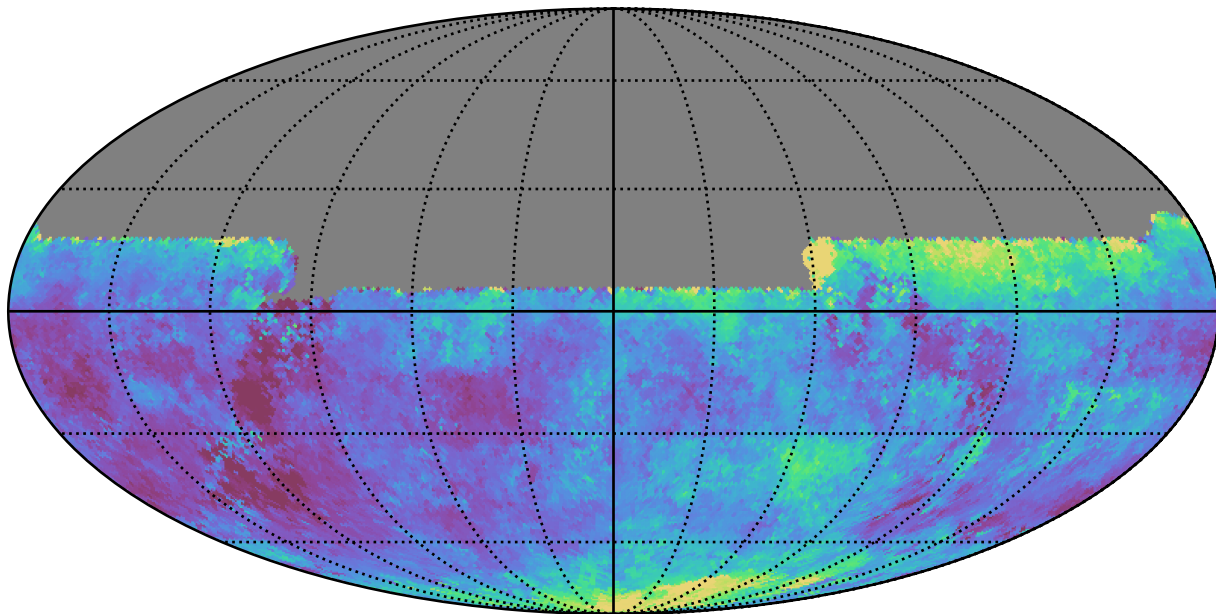
too_elab_r8_d2_giz_v3.4_10yrs All sky u band: Median seeingEff
