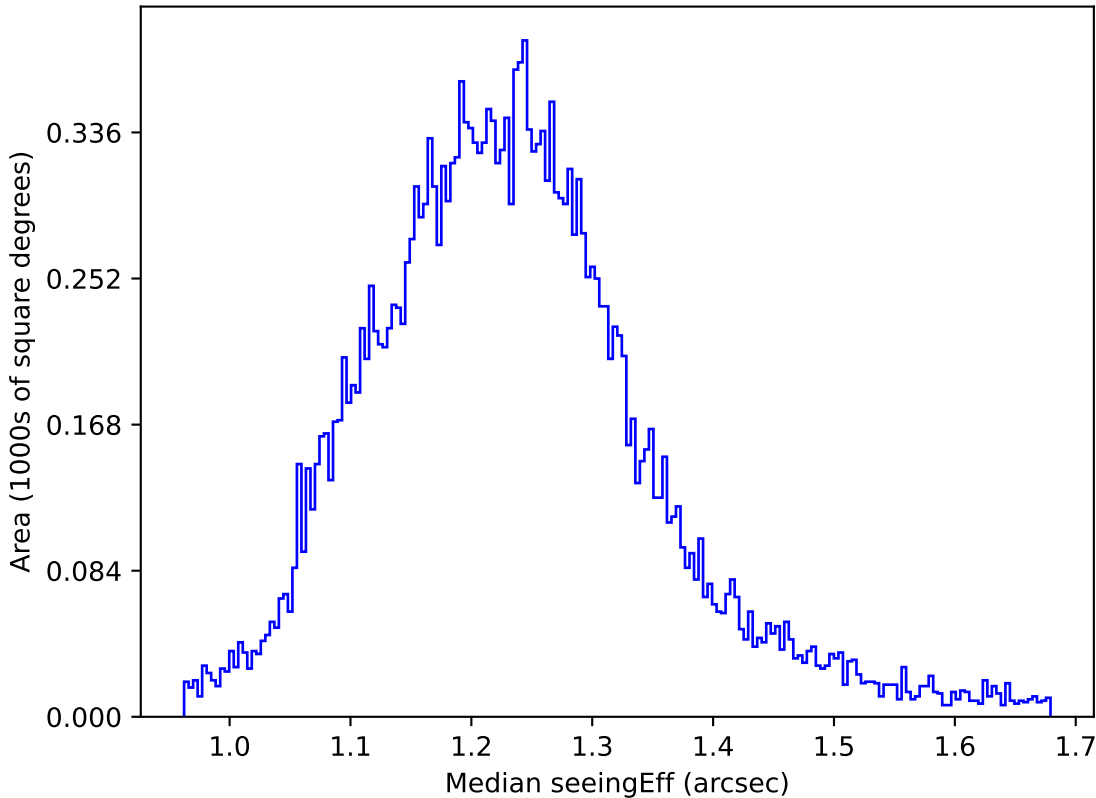
too_elab_r8_d2_giz_v3.4_10yrs All sky u band: Median seeingEff
