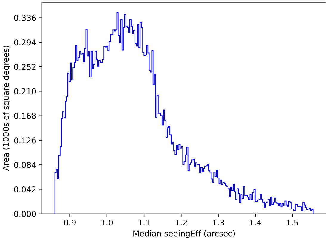
too_elab_r8_d2_giz_v3.4_10yrs All sky r band: Median seeingEff
