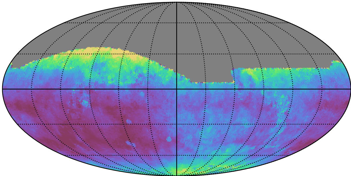
too_elab_r8_d2_giz_v3.4_10yrs All sky i band: Median seeingEff
