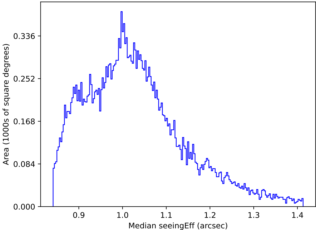
too_elab_r8_d2_giz_v3.4_10yrs All sky i band: Median seeingEff
