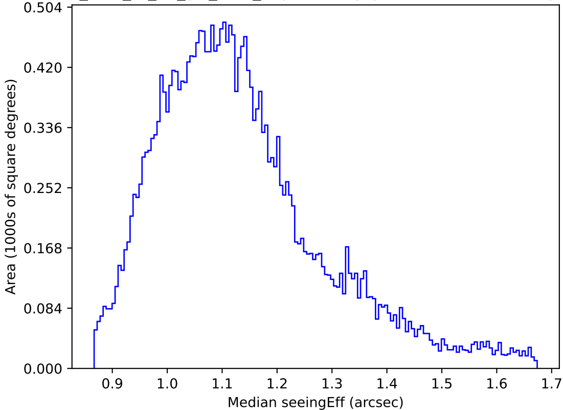
too_elab_r8_d2_giz_v3.4_10yrs All sky g band: Median seeingEff
