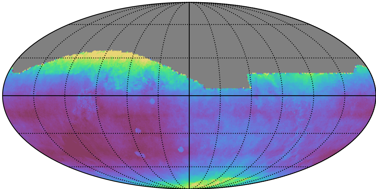
too_elab_r8_d2_giz_v3.4_10yrs All sky all bands: Median seeingEff
