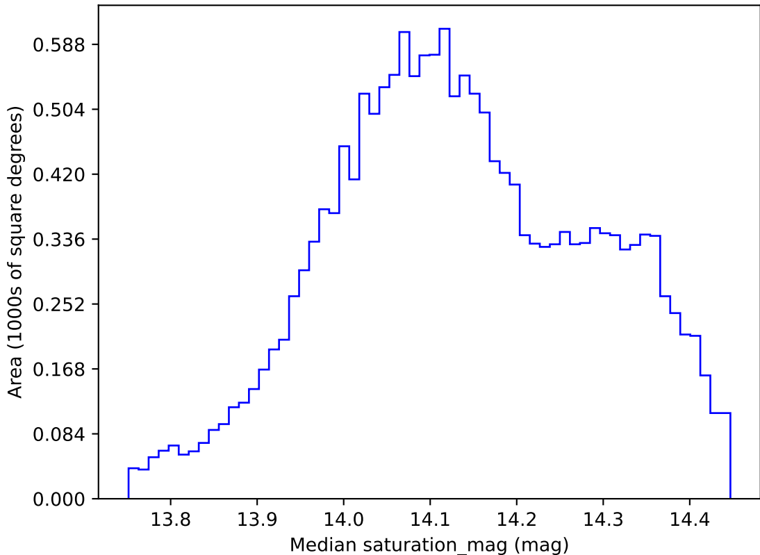
too_elab_r8_d2_giz_v3.4_10yrs WFD z band: Median saturation_mag
