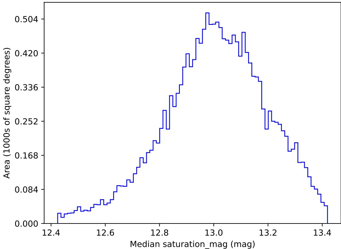
too_elab_r8_d2_giz_v3.4_10yrs WFD u band: Median saturation_mag
