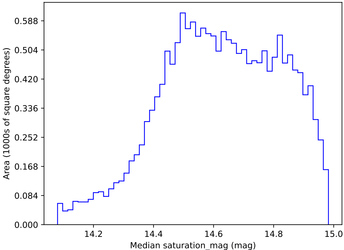
too_elab_r8_d2_giz_v3.4_10yrs WFD r band: Median saturation_mag
