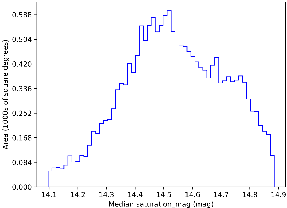
too_elab_r8_d2_giz_v3.4_10yrs WFD i band: Median saturation_mag
