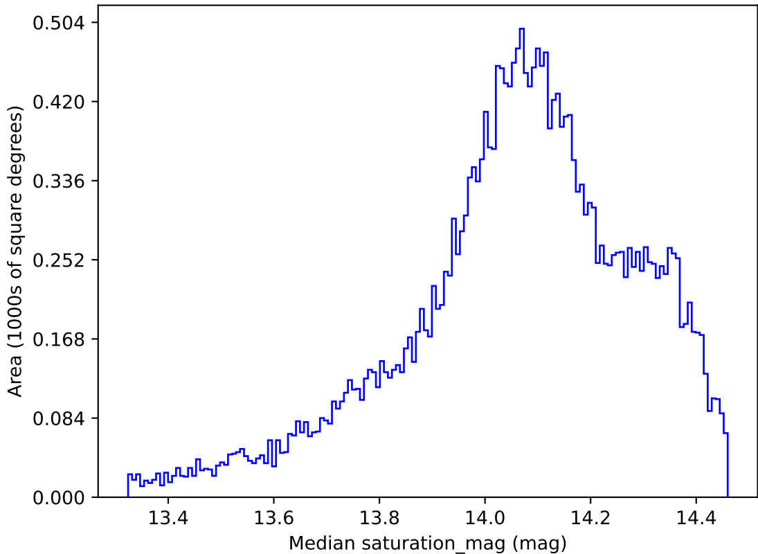
too_elab_r8_d2_giz_v3.4_10yrs All sky z band: Median saturation_mag
