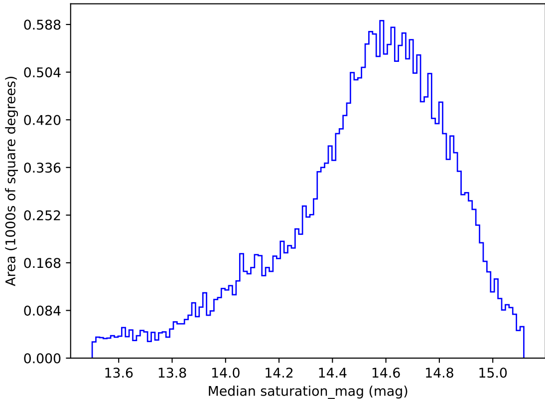
too_elab_r8_d2_giz_v3.4_10yrs All sky g band: Median saturation_mag
